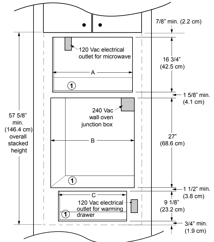
CUTOUT DIMENSIONS WITH AOMTK MICROWAVE TRIM KIT
