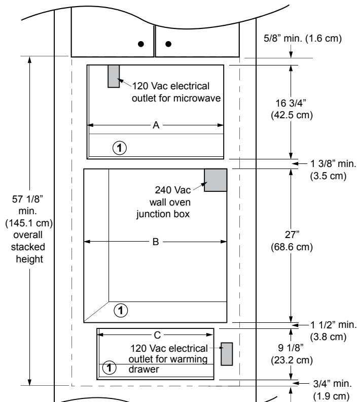
CUTOUT DIMENSIONS WITH ADMWTK MICROWAVE TRIM KIT
