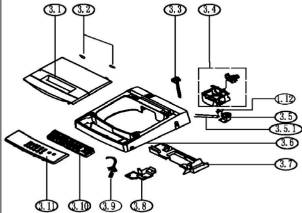
3: Top Cover Subassembly
