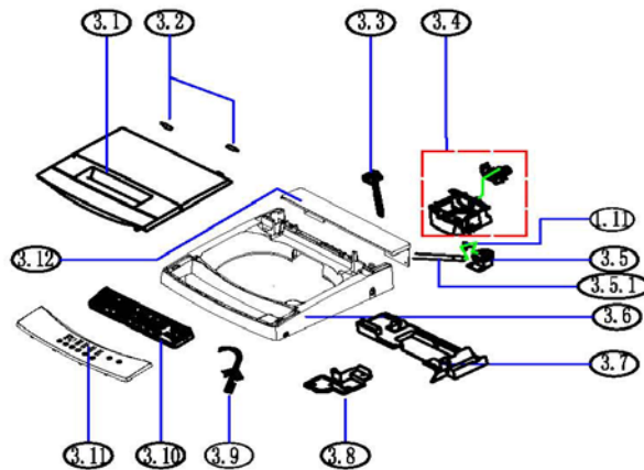
3:Top Cover Subassembly
