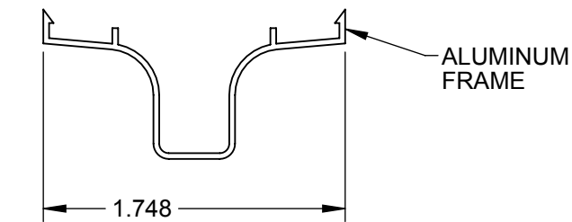
CROSS-SECTION VIEW
