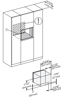
CVA7445, CVA7845, installation drawing, installation, 60 cm, Flush inset
