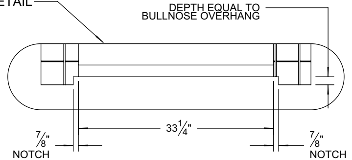
BULLNOSE NOTCH CUTOUT DETAIL
